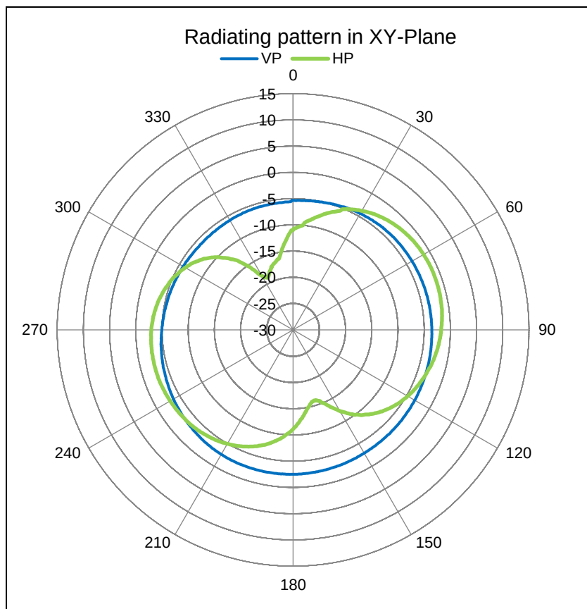
Radiation pattern polar plot (EIRP) in XY-Plane
