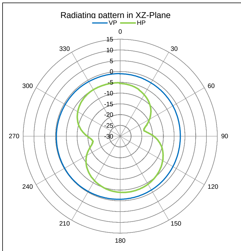
Radiation pattern polar plot (EIRP) in XZ-Plane
